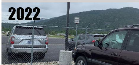
MMTS was relocated to even worse site 0.31 miles away to the airport parking lot, sandwiched between airport tarmac and airport parking. Note vehicle radiator is directly under the sensor. RATING = CRN5
