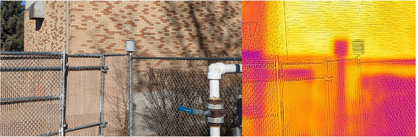
Visible and infrared photos of MMTS placement near large sunlit wall and electric power generation plant at Dillon, MT, USHCN Station at Western Montana University. Source: Anthony Watts.
