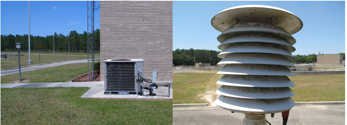
USHCN station at WWTP in Tifton, GA. Note the MMTS is directly over a sidewalk, near a brick wall, and near a/c units. This is a Class 5 station. Note in the second photo the discoloration of the MMTS, making it darker, prone to absorb more sunlight, and subsequently warmer. Source: Alan Watt.
